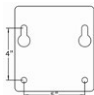
Mounting Plate (GBA-18042)
