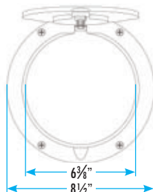
Over-sized PVB-85CVR
